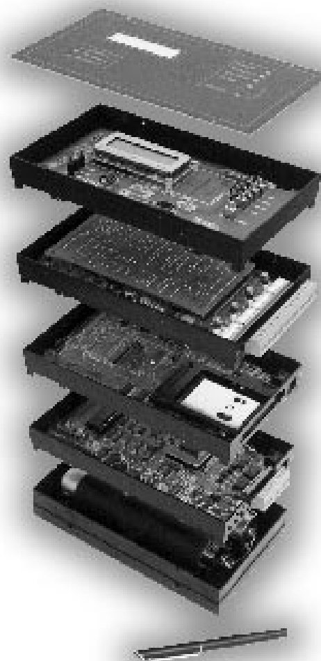
Modulogger Expanded View
